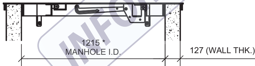
SECTION 1 SCALE 1:20
