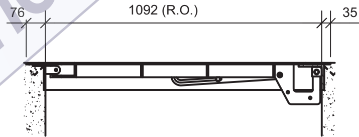
SECTION 1 SCALE 1:15
