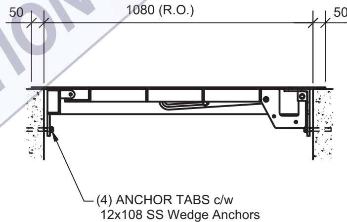
SECTION 1 SCALE 1:15
