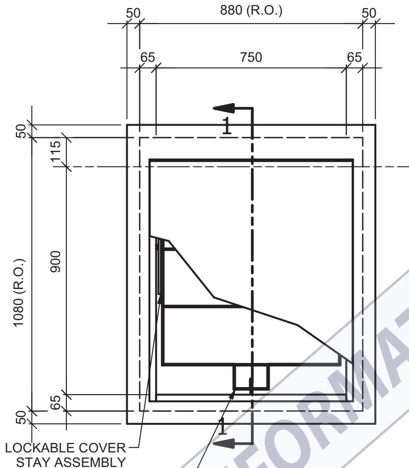
PLAN VIEW SCALE 1:15
