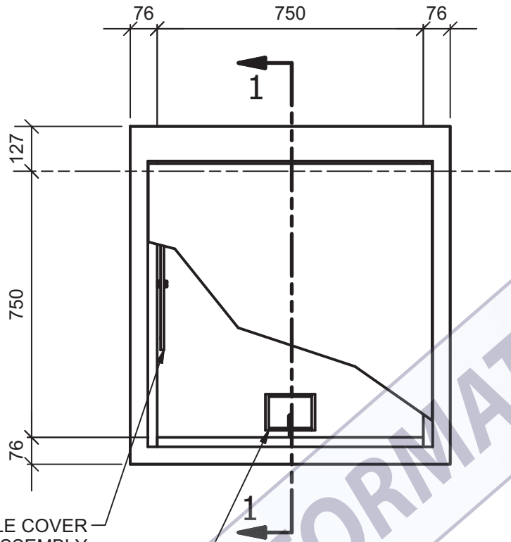
PLAN VIEW SCALE 1:15
