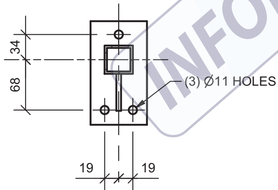
BOLT HOLE PATTERN SCALE 1:5
