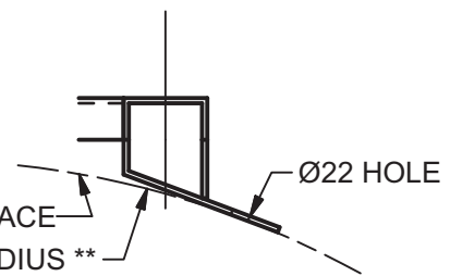
OPTION 2 CURVED MOUNTING BRACKET DETAIL SCALE 1:10
