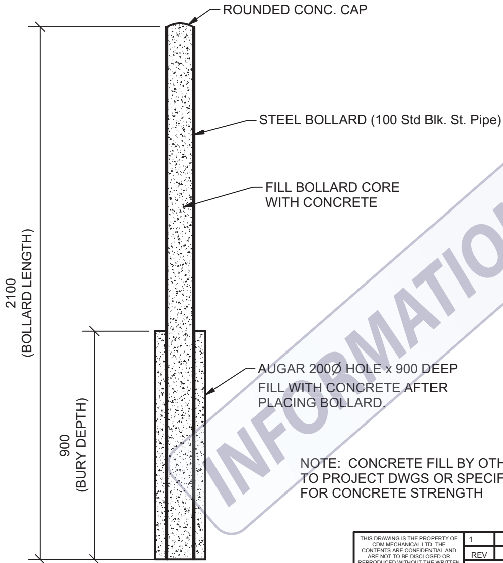
SECTION A SCALE 1:15
